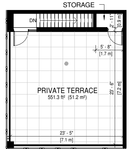
ROOFTOP LEVEL
