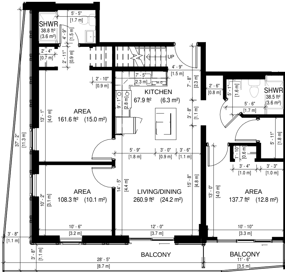
PENTHOUSE LEVEL
